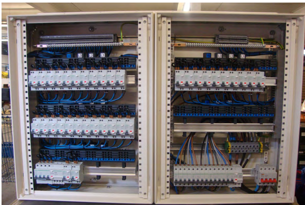
Merlin Gerin Prisma G Wall Mounted Panel
